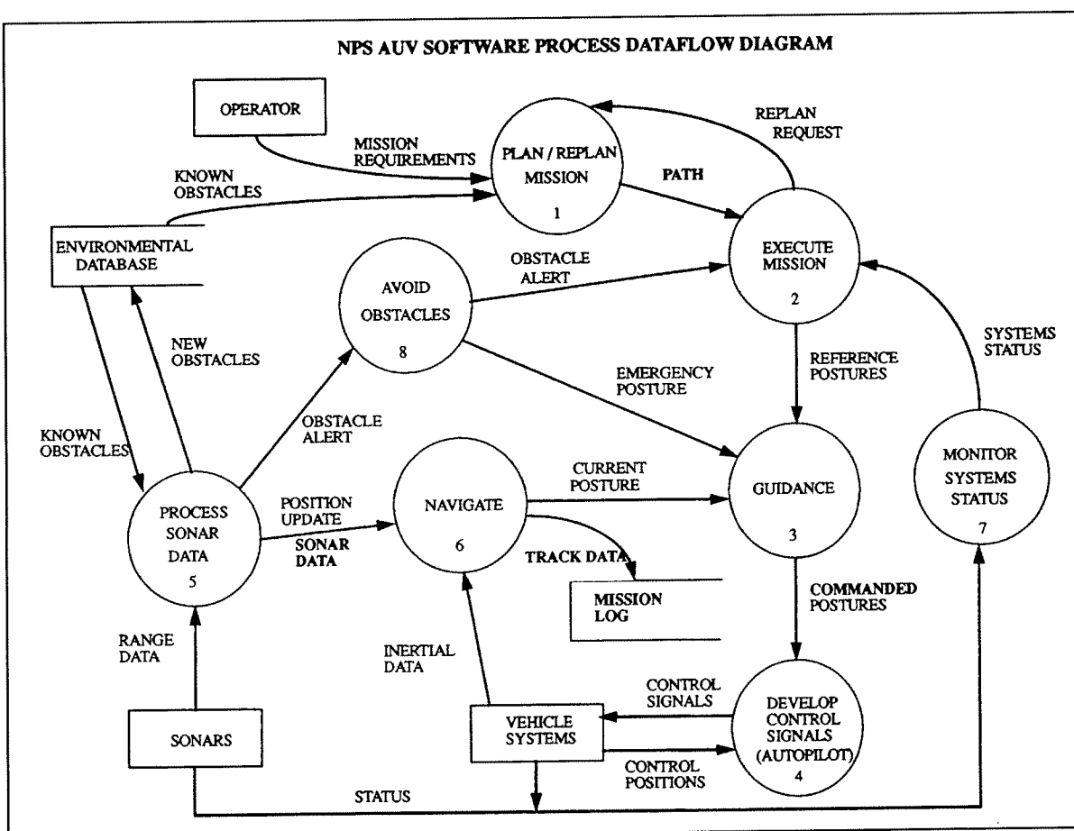
Figure 11 NPS AUV Software Process Dataflow Diagram (Courtesy of Charles A. Floyd, CDR, USN)
