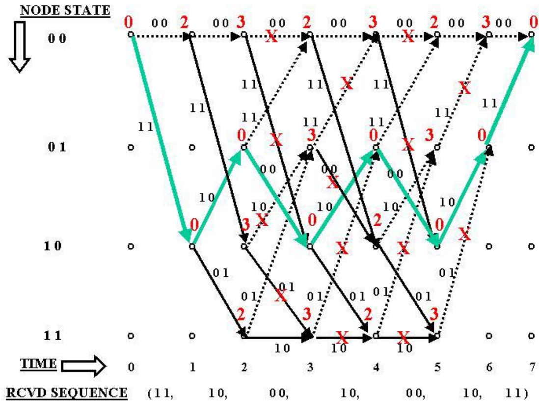
Figure 5. Viterbi Decoding Using Hamming Metric
