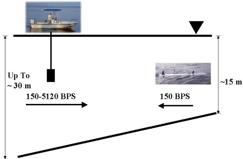
Figure 56. Converging (Decreasing Depth) Channel Geometry
