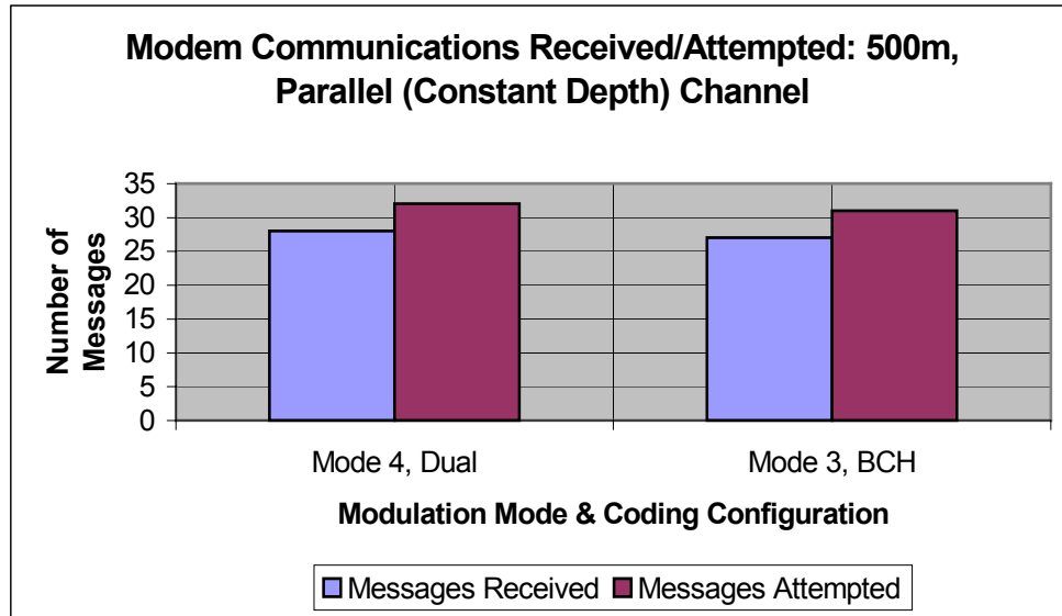
Figure 34. Message Success Data (500 Meter, Constant Depth Channel)
