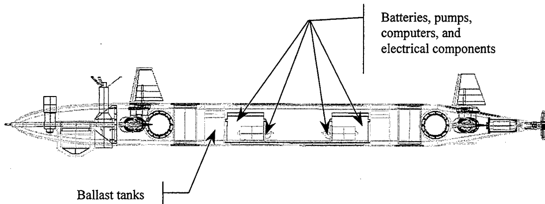
Figure II-3: New NPS AUV side view [Garibal, 1999]
